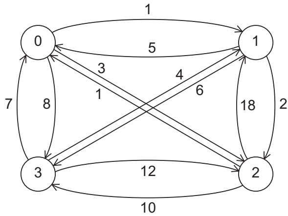
Figure 1: A four-city TSP
