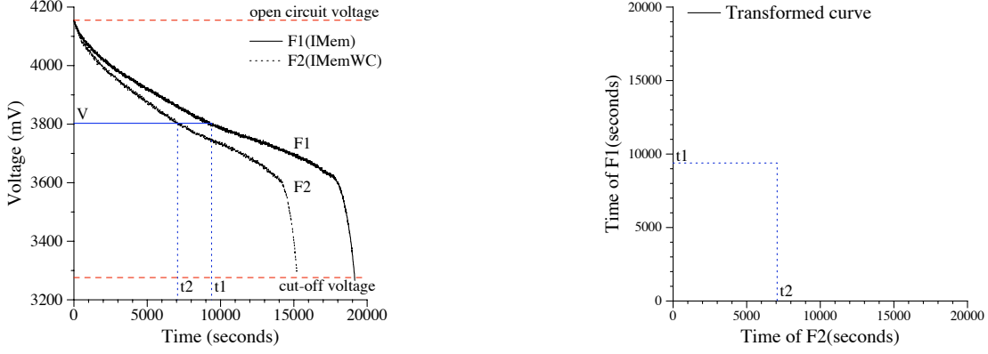
Figure 1: Timing relationship between two voltage curves of constant workloads. F_1 is the curve of the workload that is generated by repeatedly running benchmark “IMem”. And F_2 is the curve of benchmark “IMemWC”. The left graph shows that for some voltage value V , F_1 reaches V at time t_1 and F_2 reaches V at time t_2 . The right graph shows the linear relationship between t_1 and t_2 for any V .
